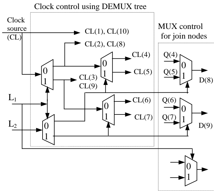
Figure 4: A hierarchical clock gating logic for DTS(2)
