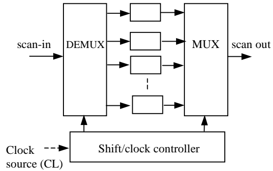
Figure 1b: Fully parallel scan-path
