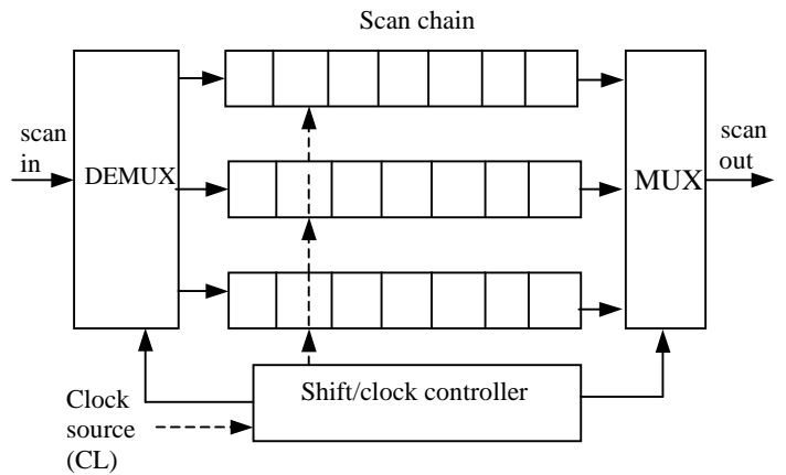
Figure 1c: Multiple parallel scan-path
