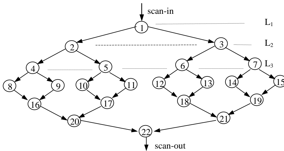
Figure 2c: DTS(3); # FFs (f) = 22
