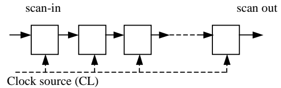
Figure 1a: Linear scan-path
