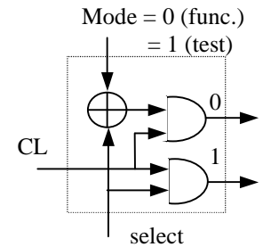
Figure 8: DEMUX
