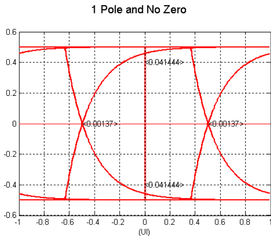
Figure 7. A one-pole model: Eye-diagram.
